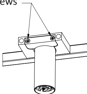
Adjustment Screws
